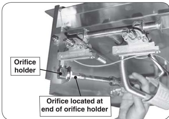
Fig. 22-2 Orifice location
