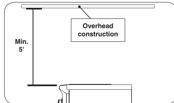
Fig. 9-1 Overhead requirements
